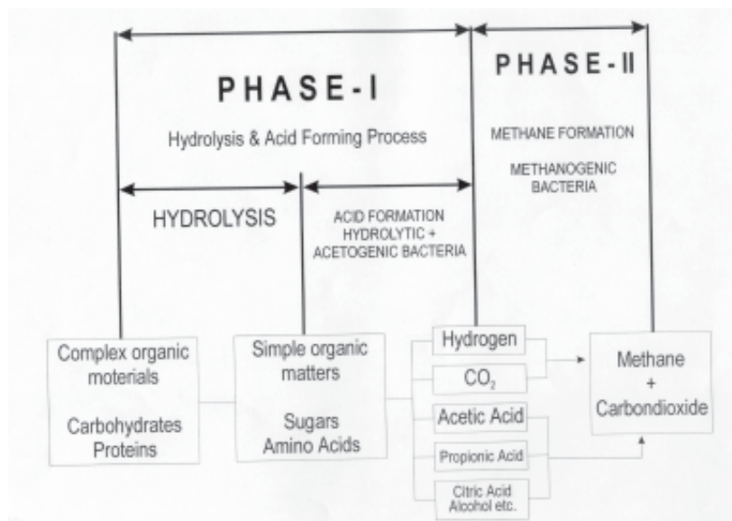
Figure - 3: Disphasic Digestion
